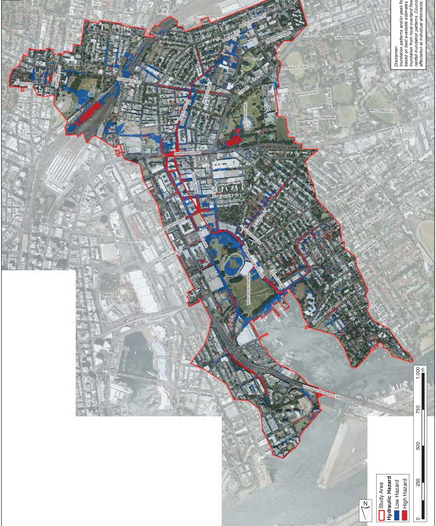
FIGURE 17 HAZARD CATEGORIES 5% AEP DESIGN FLOOD EVENT
