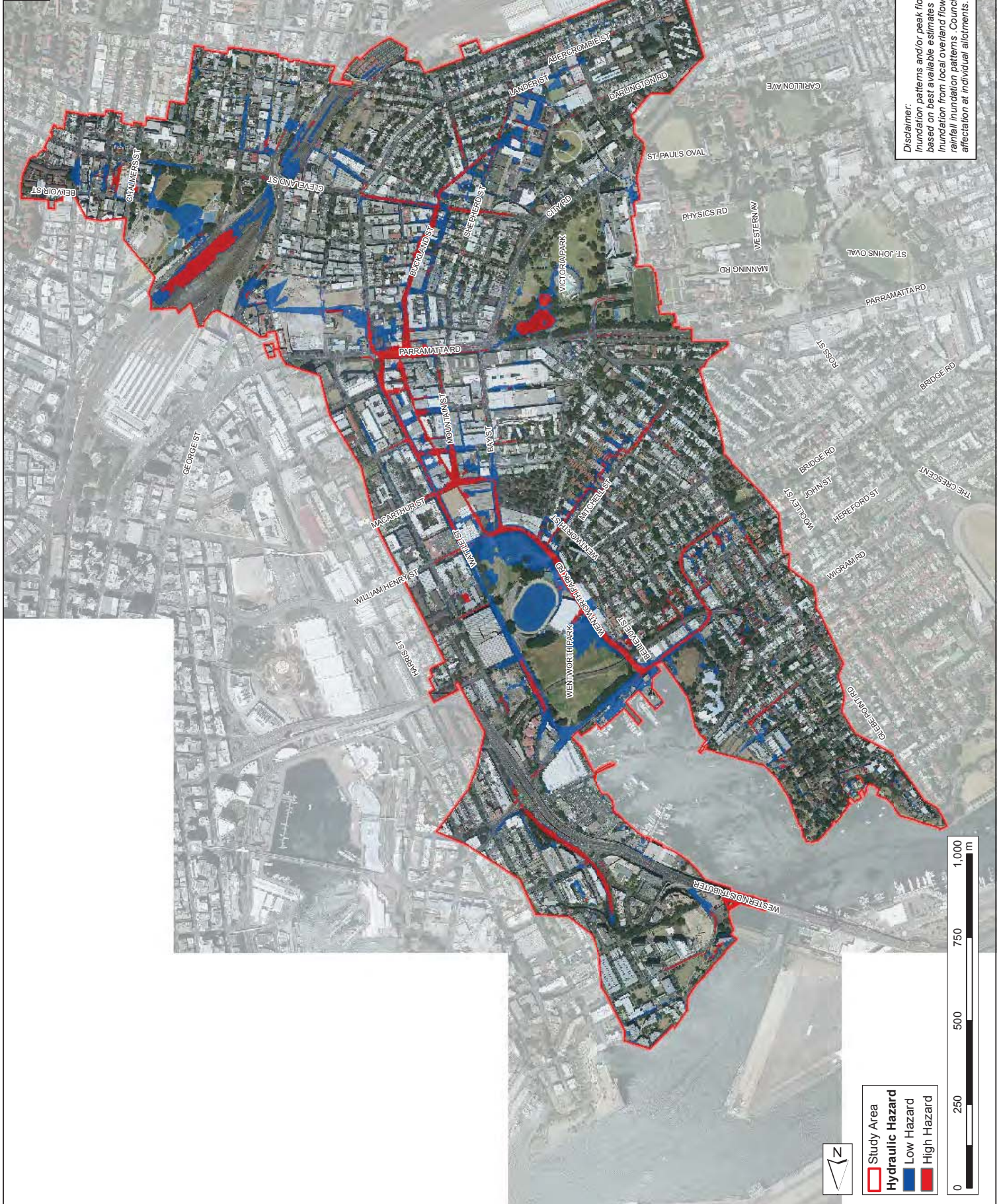
FIGURE 18 HAZARD CATEGORIES 2% AEP DESIGN FLOOD EVENT
